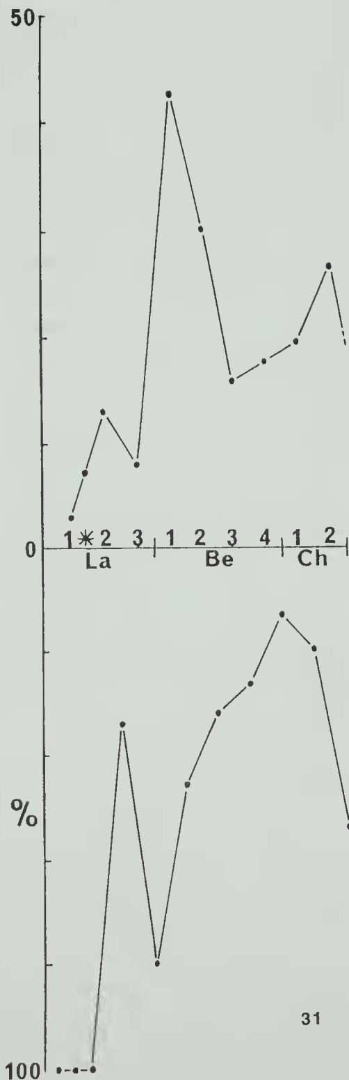
Figure 31. Diversity of Lancefieldian to Chewtonian graptolites; upper graph shows number of species at each horizon, lower graph the percentage change over between divisions; data from O.P. Singleton (pers. comm.) modified only to include new forms and synonymies in the Bendigonian; Lancefieldian La 1.5 is shown with an asterisk.
